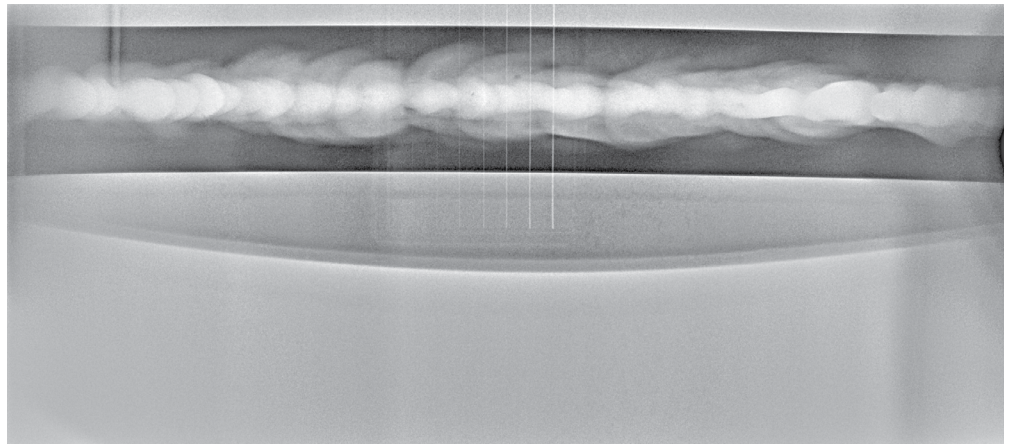
6 inch steel pipe, 6mm wall thickness, shot with YXLON ECO200DS
